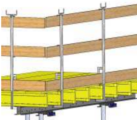
Slab formwork
