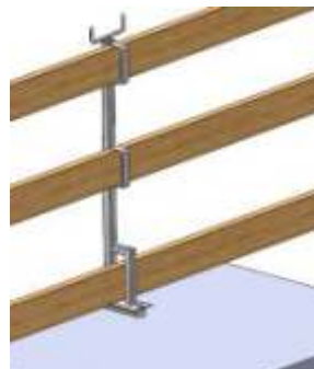
Fixing with dowel and screw
